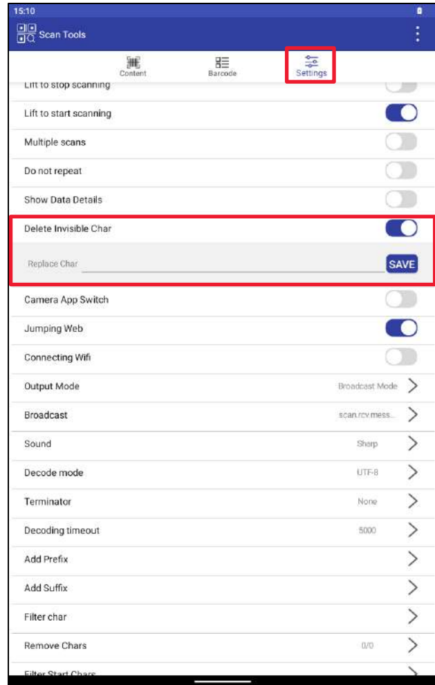
Рисунок 114. Settings. Delete Invisible Char → Replace Char
